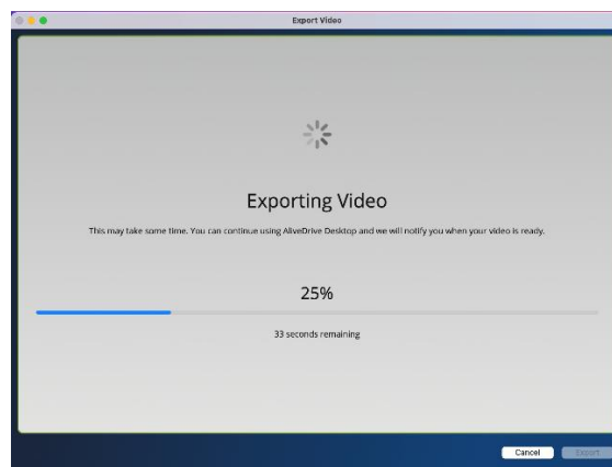
Figure 21 - Export Progress
