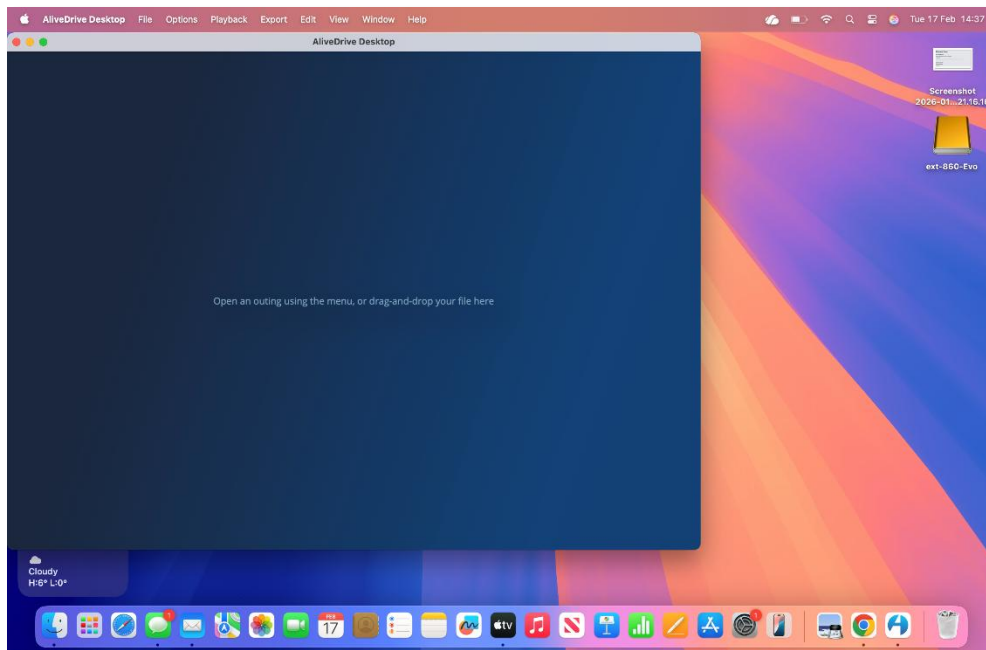
Figure 3 – Application Launch
