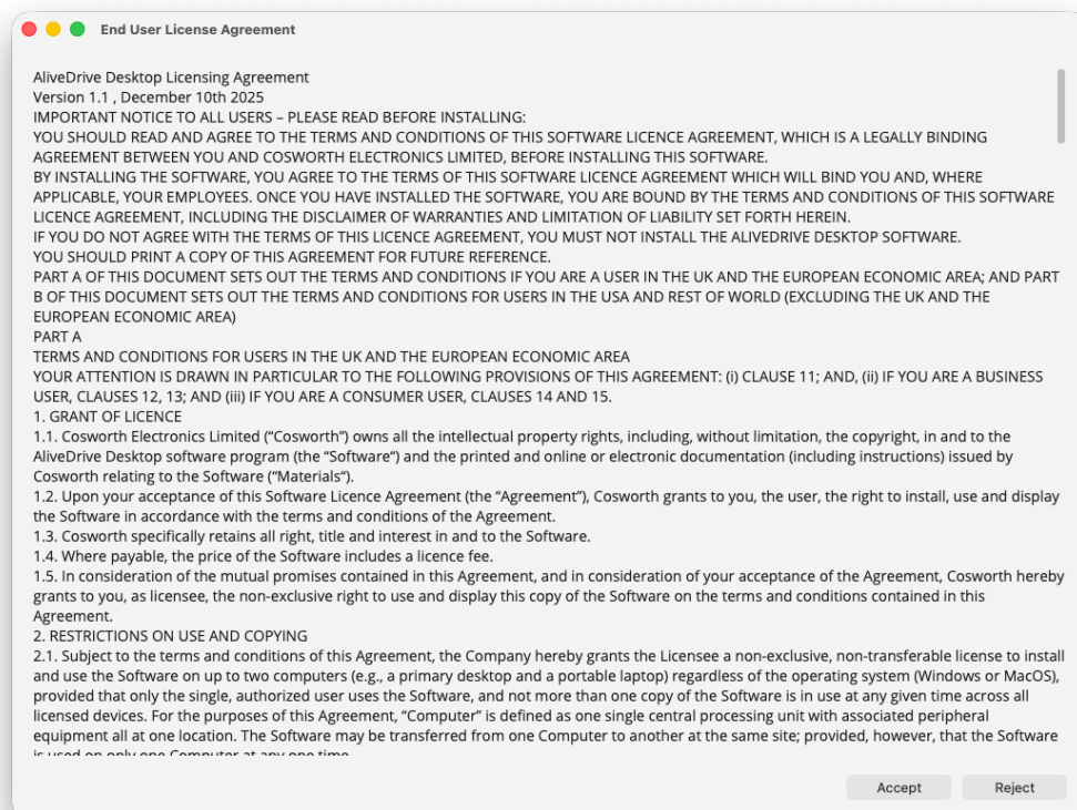
Figure 2 - Licence Agreement
