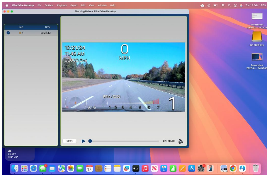
Figure 4 - Light Mode
