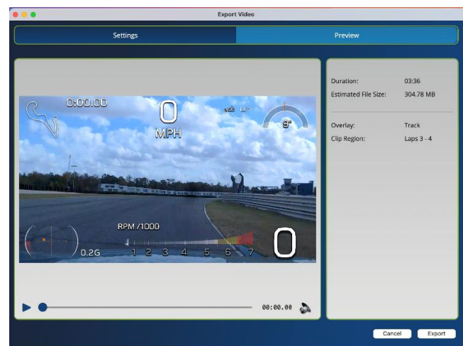
Figure 18 - Export Preview
